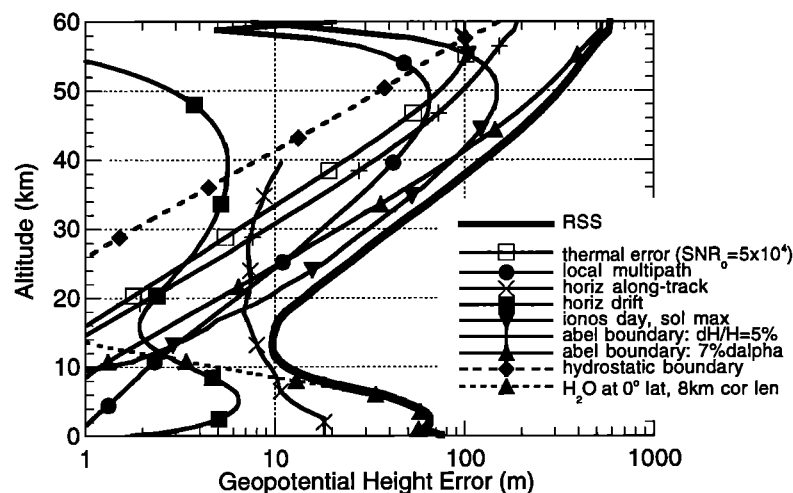
Figure 11. Summary of geopotential height errors versus height. Thermal error, 1 s \text{SNR}_0 = 5 \times 10^4 ; local multipath, 10 mm rms spread over 0.01 Hz; horizontal refractivity structure, along track from simulation and horizontal motion of ray path tangent point from tropospheric and stratospheric climatologies near 30°S for June–July–August; ionosphere error, daytime, solar maximum conditions; Abel boundary error, 7% in \alpha , 5% in H_\alpha ; hydrostatic boundary error, 5 K; tropospheric water vapor, 0° latitude with 8 km vertical correlation length based on Figure 22.
