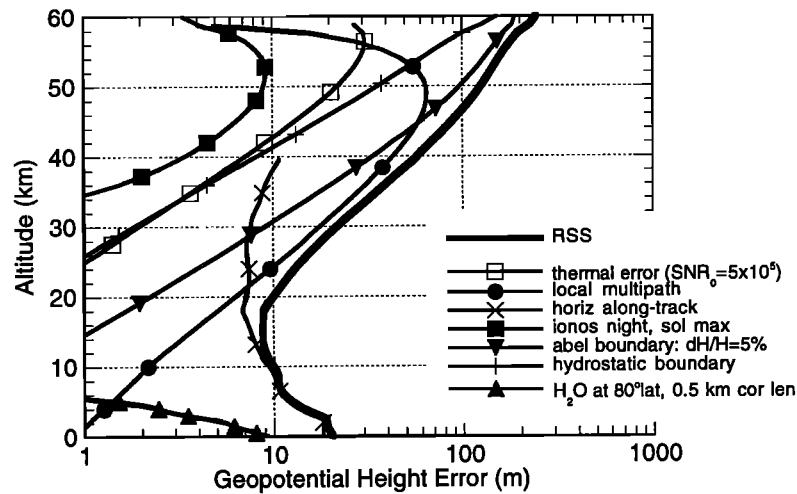
Figure 14. Summary of geopotential height errors versus height. Thermal error, 1 s SNR=5x10 5 ; local multipath, 10 mm rms spread over 0.01 Hz; horizontal refractivity structure, along track from simulation; ionosphere error, nighttime, solar maximum conditions; Abel boundary error, 5% in H_{\text{ref}} ; hydrostatic boundary error, 5 K; tropospheric water vapor, 80° latitude with 0.5 km vertical correlation length based on Figure 22.
